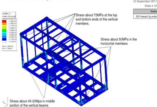
VonMises Stress During Acceleration
